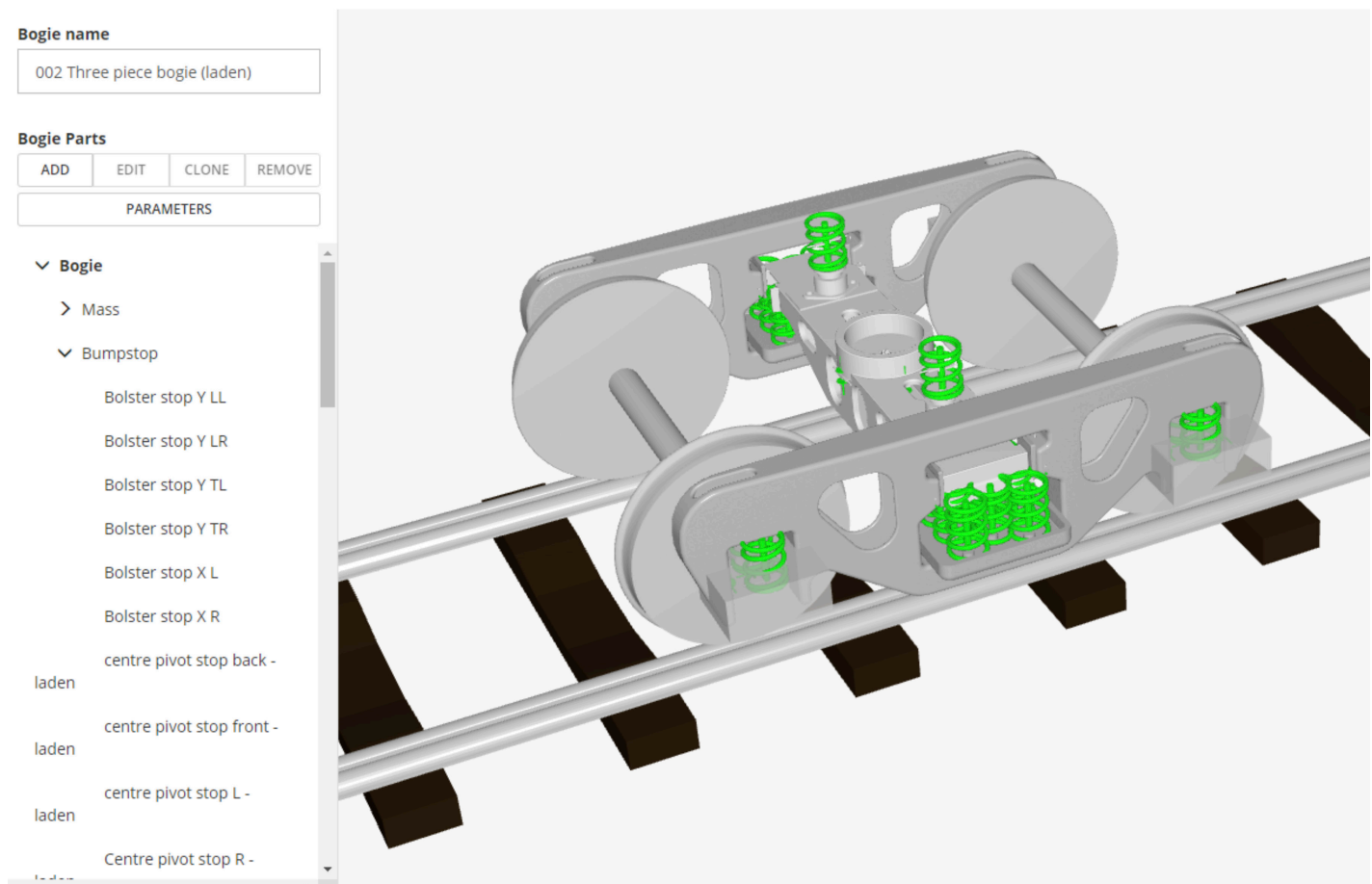
Figure 2.1 Snapshot of DigitalTrains™ Bogie builder
