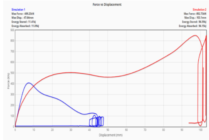
Figure 3.5 Comparison of force-stroke diagrams on curve with those on a straight track.
