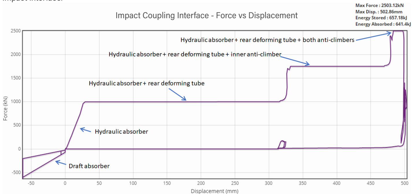
Figure 3.10 Total force deflection diagram at impact interface on 200m radius curve at 25km/h
