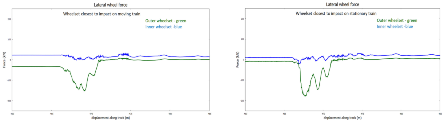
Figure 3.6 The lateral wheel forces on moving and stationary vehicles.
