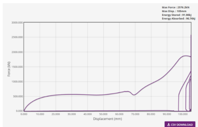
Figure 3.4 Stroke diagrams for inner and outer side buffers
