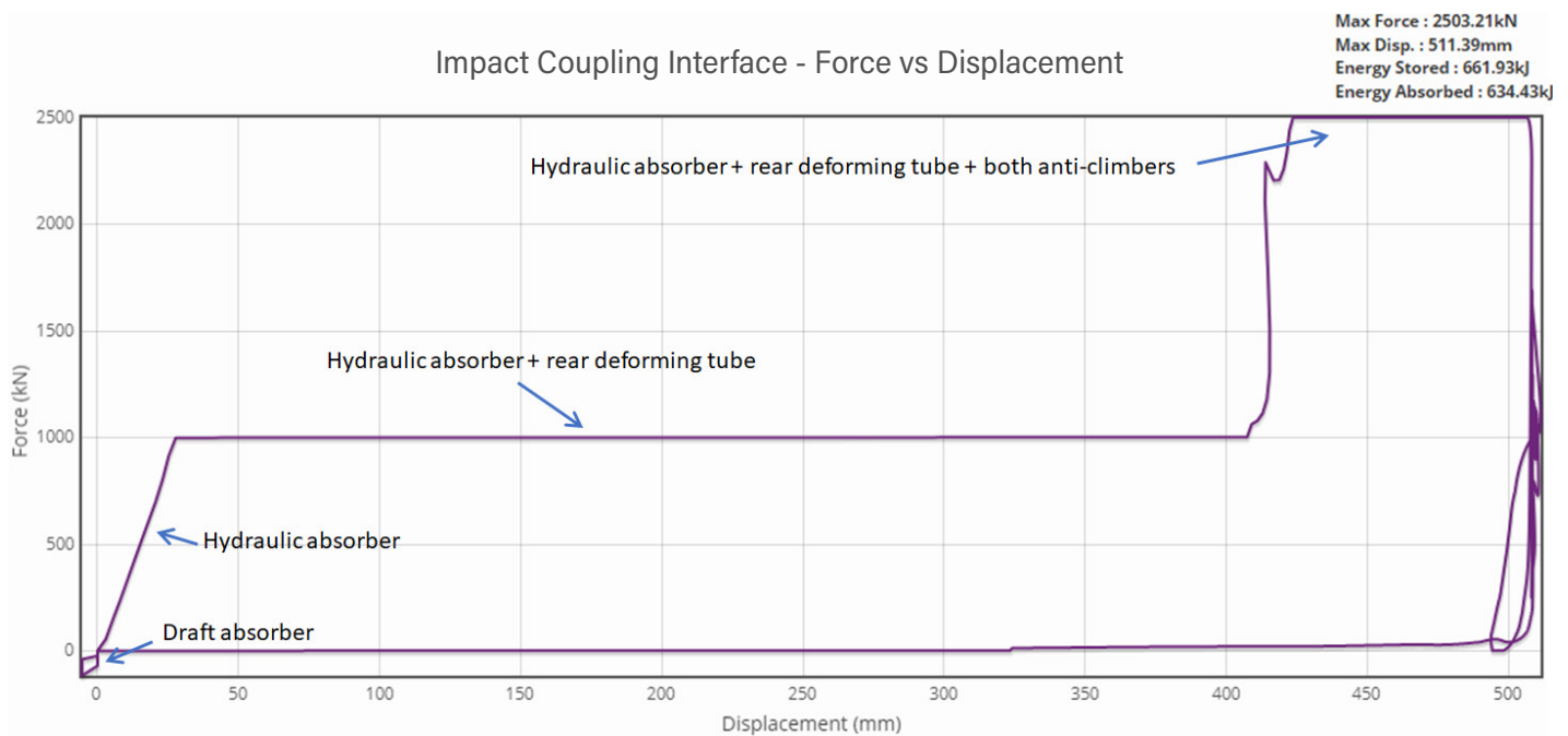
Figure 3.11 Total force deflection diagram at impact interface on 200m radius curve at 25km/h
