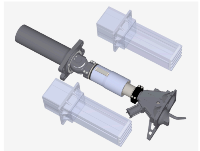
Figure 3.7 Auto Coupler interface geometry
