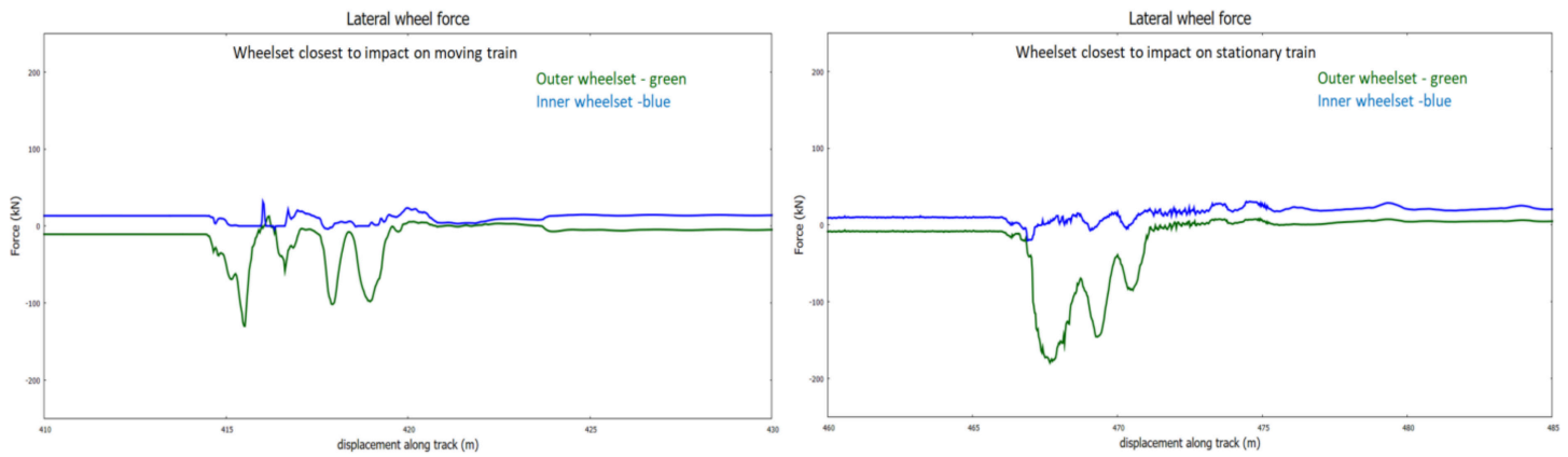
Figure 3.12 Total force deflection diagram at impact interface on 200m radius curve at 25km/h
