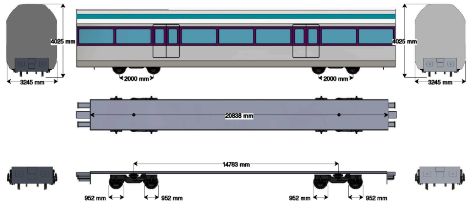
Figure 2.2 Vehicle geometry
