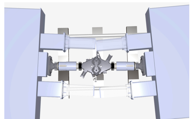
Figure 3.9 Alignment of Anti-Climbers at point of contact
