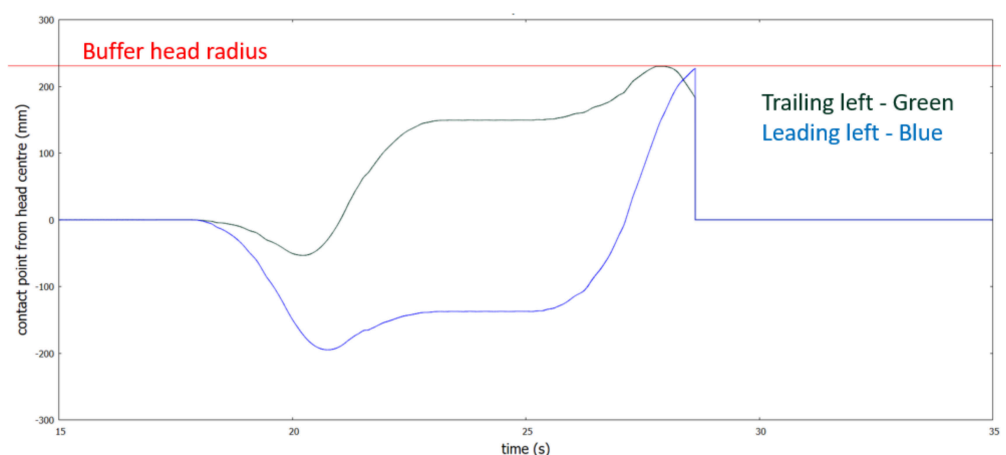
Figure 2.4 Lateral displacement of contact between buffer heads
