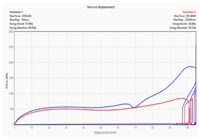
Figure 3.5 Comparison of force-stroke diagrams on curve with those on a straight track.
